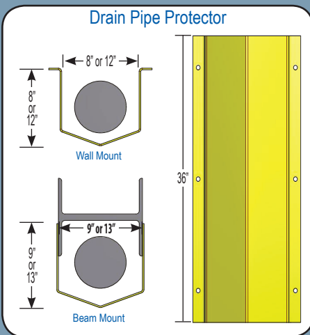
Figure 2: Dimensions of the Drain Pipe Protector
