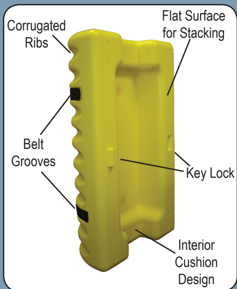
Figure 2: Column [I-Beam] Protector design highlights
