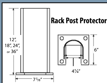
Figure 2: Dimensions
